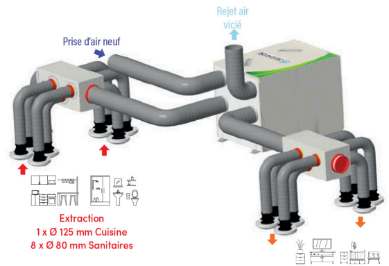
Installation verticale
